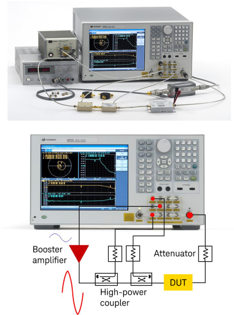
Figure 5. Configuration example using direct receiver access
