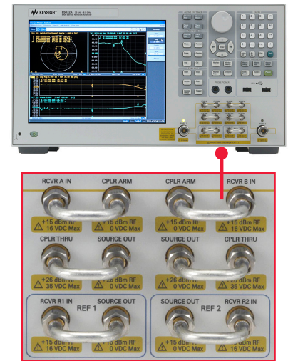
Figure 1. Jumpers on front panel
