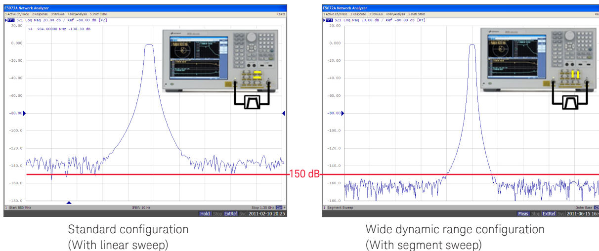
Figure 13. Dynamic range of forward measurements is improved with the configured wide dynamic range
